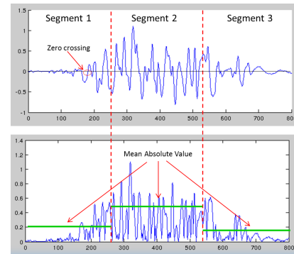
Figure 5. A typical sEMG signal segmented into 3 parts. The zero-crossings are indicated in the top figure. The rectified signal and the MAVs of the segments are shown in the bottom figure.
