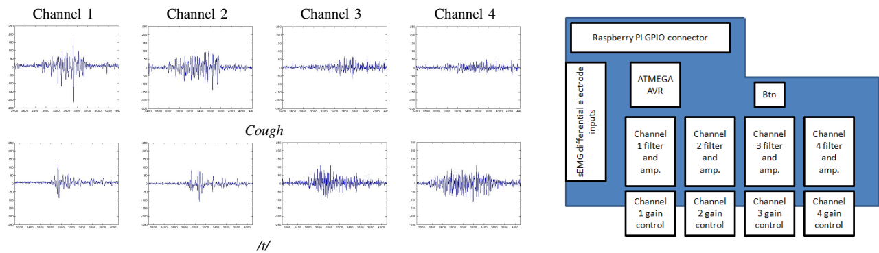
Figure 2. a) Four channels of sEMG signals for gestures Cough and /t/ ; and b) Basic diagram of the custom PCB for the ECHO-OREAD device.
