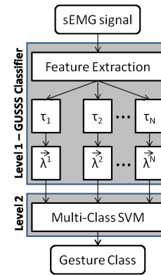
Figure 4. Proposed framework for the Hierarchical GUSSS Classifier used in the ECHO-OREAD.
