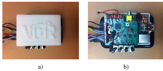
Figure 1. ECHO device depicted from two top angles: a) with and b) without the case cover.
