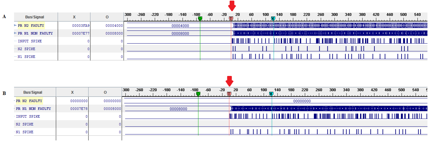
Fig. 6: Chipscope results on real hardware (Nexys-4 Artix-7 FPGA board): Fault of 100% ( PR of all the synapses associated with neuron N2 are intentionally lowered from 0.5) is induced on synapses connected to N2 at the trigger point T (A) Partial fault ( PR(t_0) = 0.25 )(B) Catastrophic fault ( PR(t_0) = 0.0 ). The PR values of faulty synapse lowers to zero in the presence of catastrophic fault whereas has a moderate value in the presence of partial fault. Also the spikes produced by N2 ceases in the case of a catastrophic fault(B), whereas has a moderate value in the presence of partial fault(A).
