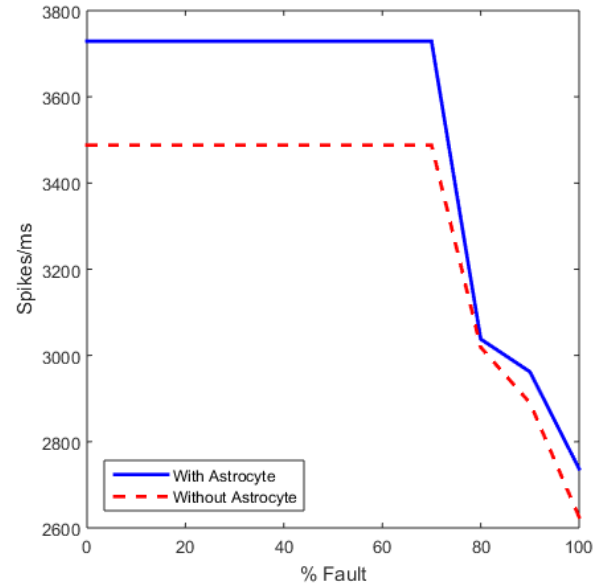
Fig. 7: Average firing rate of self repairing unit an astrocyte and without an astrocyte. It can be seen that the spike rate is higher in all cases in the presence of astrocyte.
